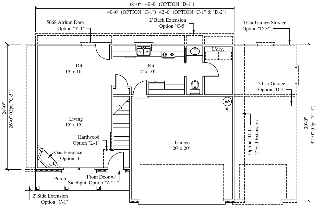
Floor Plan
