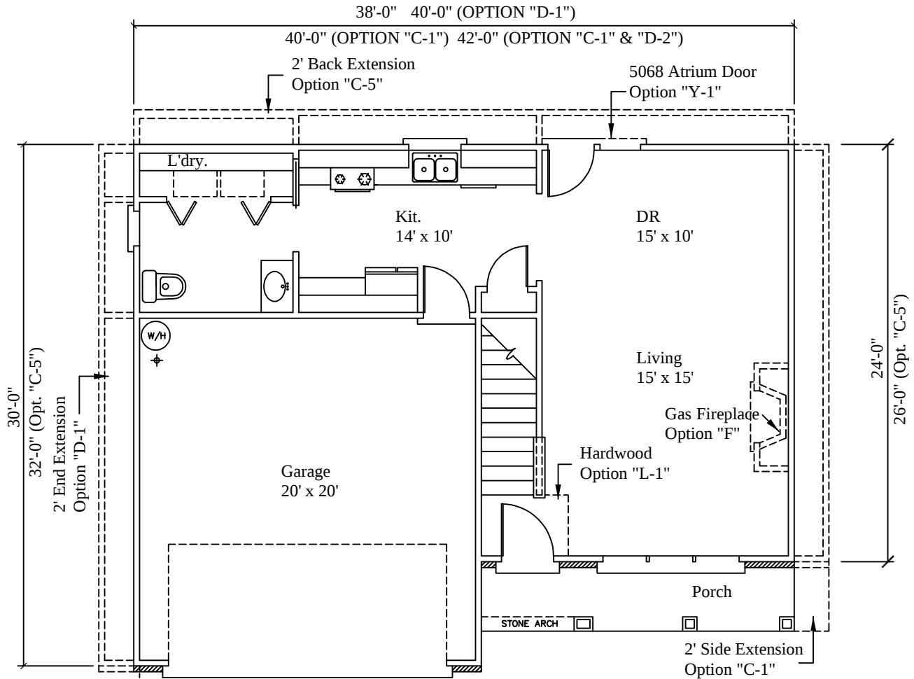
Floor Plan
